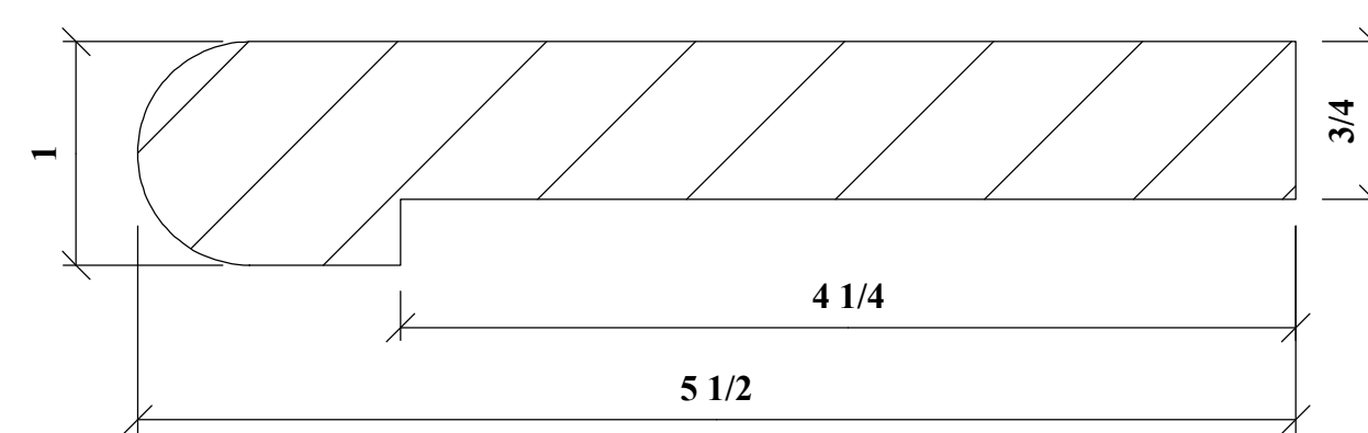
Pine Landing Tread (Match Treads)
