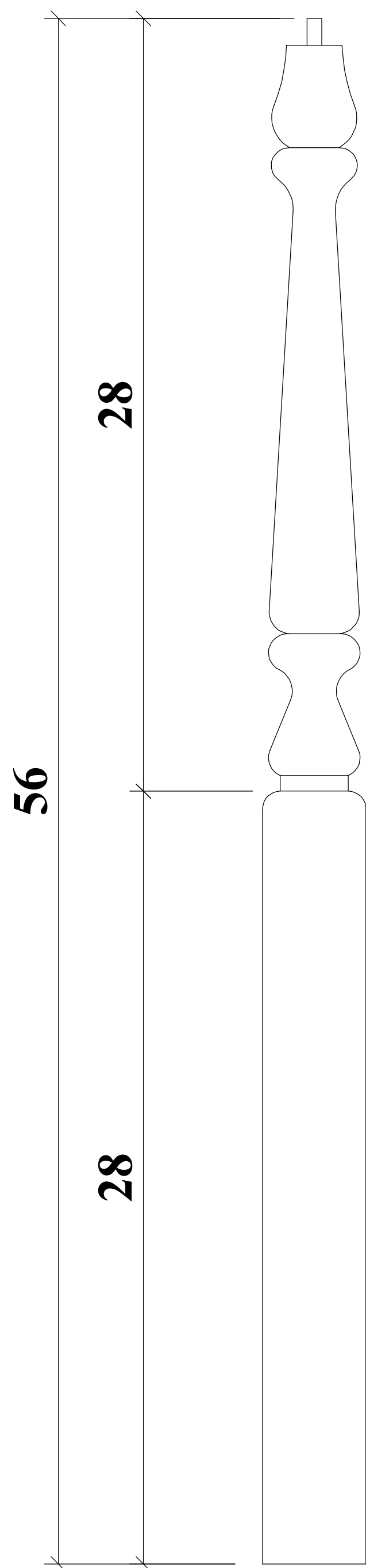
#4815 - Regency Newel Pin Top
