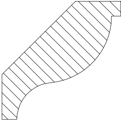
Crown 6-1 15/16" x 2 13/16"
