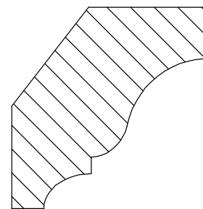
Crown 14-5 15/16" x 2 1/16"
