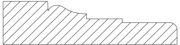
Casing 9-2 7/8" x 3 1/2"
