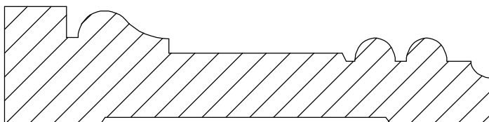
Casing 11-7 7/8" x 3 5/8"
