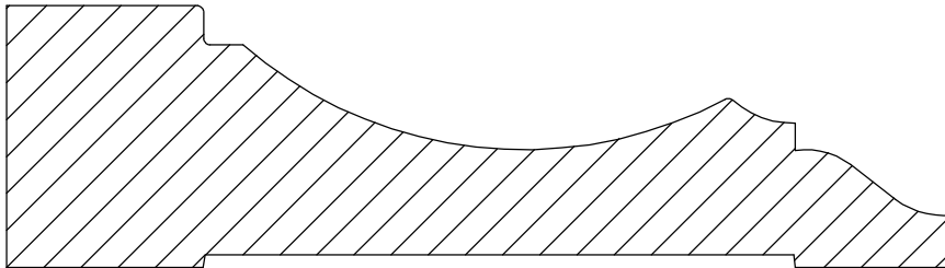
Casing 8-3 1 1/4" x 4 1/2"
