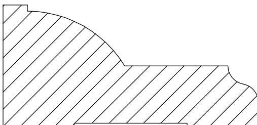
Casing 8-5 1 1/4" x 2 5/8"
