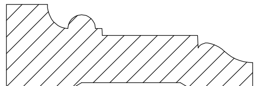
Casing 10-6 7/8" x 2 5/8"
