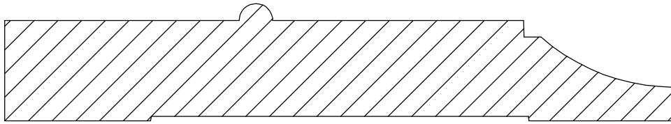
Casing 9-1 7/8" x 5"
