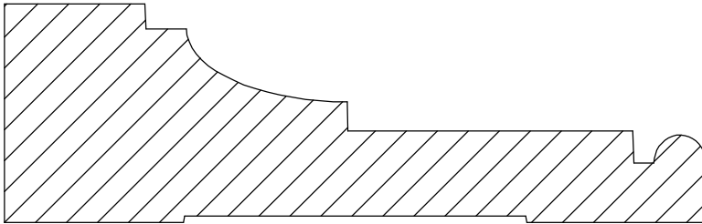
Casing 1-3 1 1/4" x 4"
