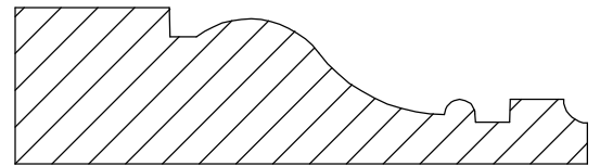
Casing 10-4 3/4" x 2 3/4"
