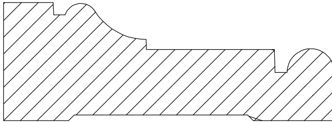
Casing 3-3 1 1/4" x 3 1/2"
