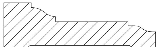
Casing 6-7 13/16" x 2 3/4"
