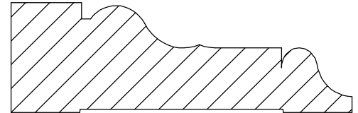
Casing 3-2 13/16" x 2 1/2"
