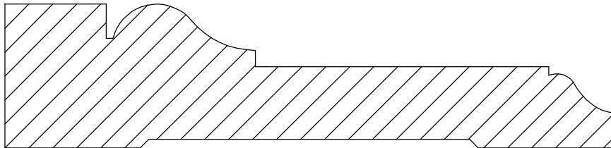
Casing 4-3 1 1/16" x 4 1/2"
