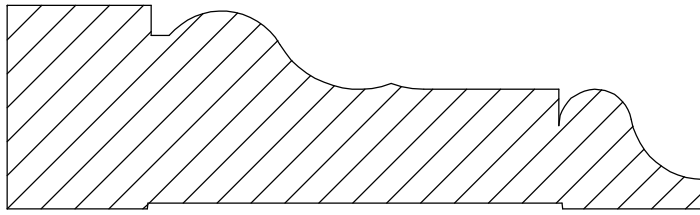
Casing 3-1 1 1/16" x 3 5/8"
