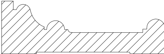
Casing 9-3 1 1/8" x 3 1/2"
