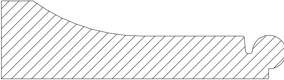
Casing 11-1 1 3/8" x 5"
