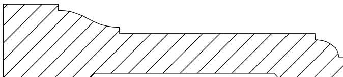
Casing 7-5 3/4" x 3 1/2"
