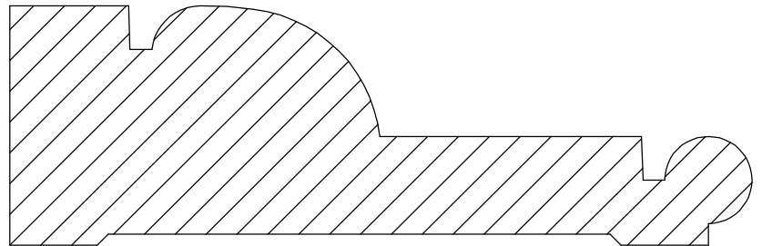
Casing 7-2 1 3/8" x 4 1/4"
