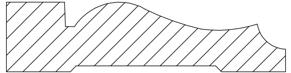
Casing 10-2 3/4" x 3"
