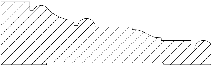
Casing 1-5 1 1/8" x 3 3/4"
