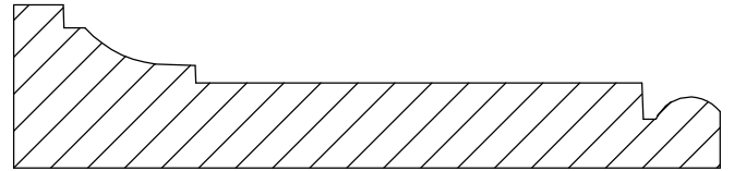
Casing 1-2 13/16 x 3 3/8
