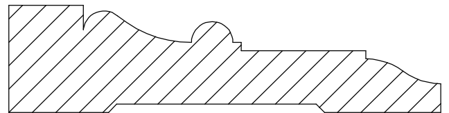
Casing 1-4 13/16" x 3 1/4"
