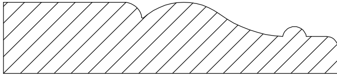
Casing 10-1 3/4" x 3 1/2"
