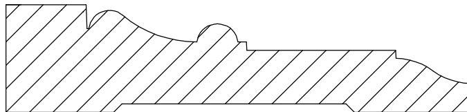
Casing 11-5 13/16" x 3 1/2"
