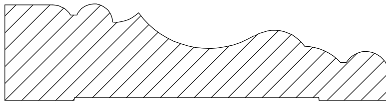
Casing 6-3 1" x 4"
