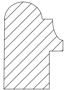
Backband 15-4 1 1/16" x 1 5/8"
