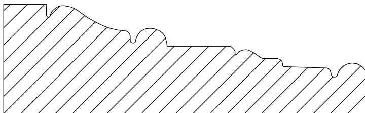
Casing 3-5 1 1/8" x 3 5/8"
