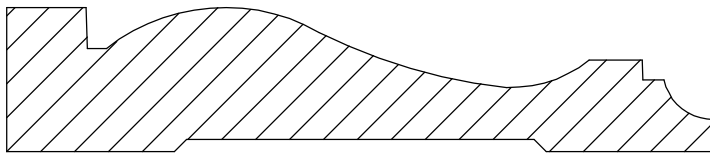
Casing 9-5 3/4" x 3 11/16"
