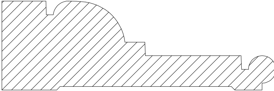
Casing 7-1 1 5/8" x 5"
