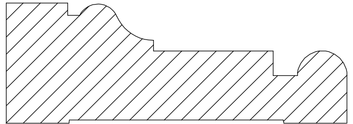
Casing 2-2 1 1/4" x 3 1/2"
