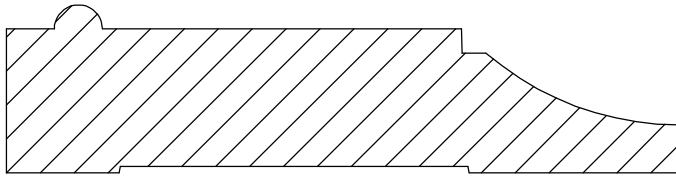
Casing 2-3 7/8" x 3 1/2"
