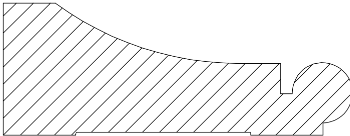
Casing 11-2 1 3/8" x 3 5/8"
