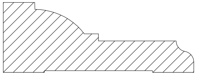
Casing 8-2 1 1/4" x 3 3/8"
