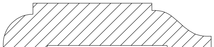
Casing 4-6 3/4" x 3 1/2"
