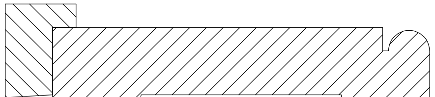
Casing 8-4 1" x 4 1/2"
